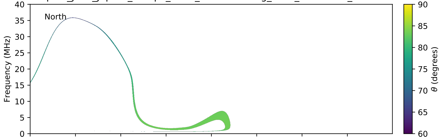
expres_juno_jupiter_europa_isaac_lossc-wid1deg_3kev_20160724_v01.cdf
