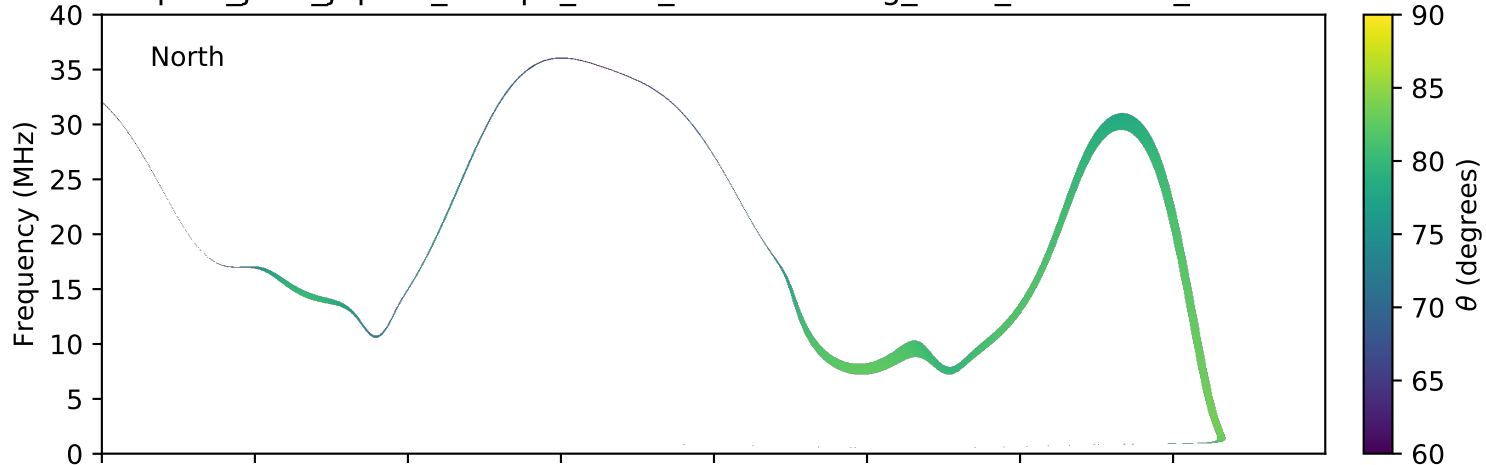
expres_juno_jupiter_europa_isaac_lossc-wid1deg_3kev_20160720_v01.cdf
