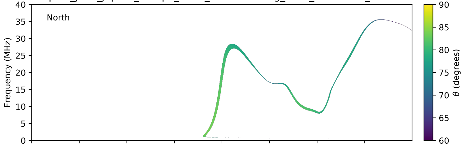
expres_juno_jupiter_europa_isaac_lossc-wid1deg_3kev_20160719_v01.cdf
