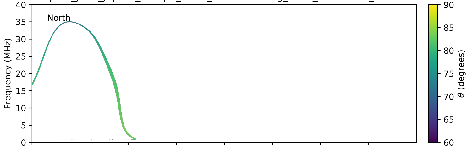
expres_juno_jupiter_europa_isaac_lossc-wid1deg_3kev_20160717_v01.cdf
