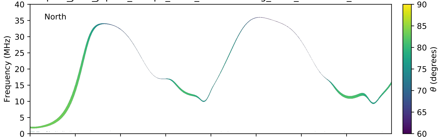
expres_juno_jupiter_europa_isaac_lossc-wid1deg_3kev_20160716_v01.cdf
