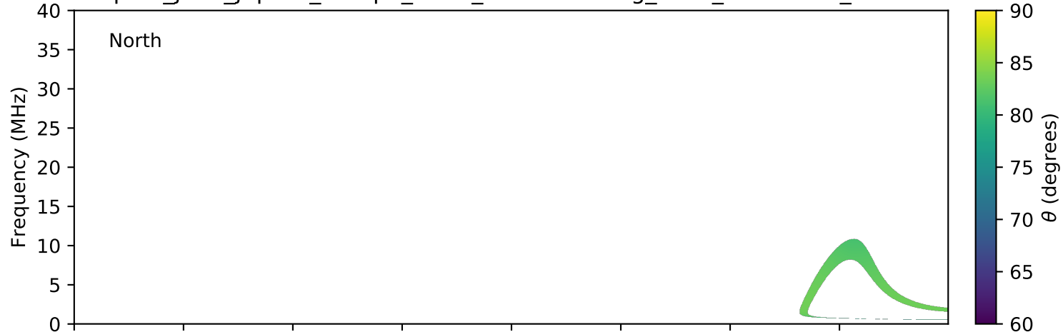
expres_juno_jupiter_europa_isaac_lossc-wid1deg_3kev_20160715_v01.cdf
