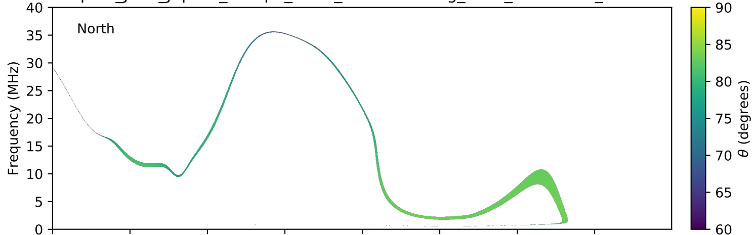
expres_juno_jupiter_europa_isaac_lossc-wid1deg_3kev_20160713_v01.cdf
