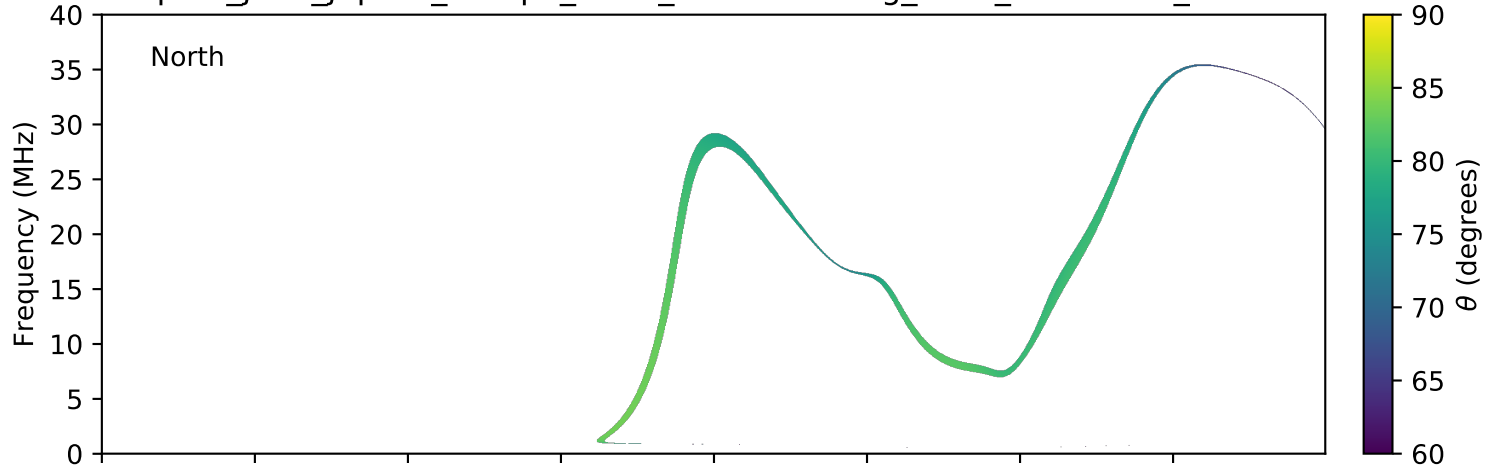
expres_juno_jupiter_europa_isaac_lossc-wid1deg_3kev_20160712_v01.cdf
