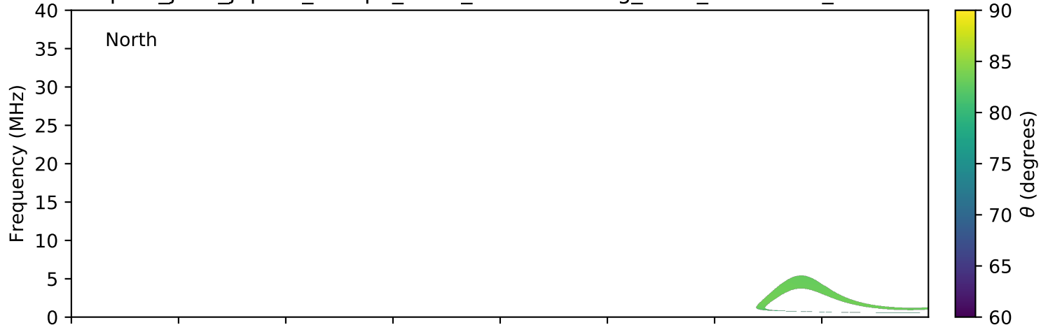
expres_juno_jupiter_europa_isaac_lossc-wid1deg_3kev_20160708_v01.cdf
