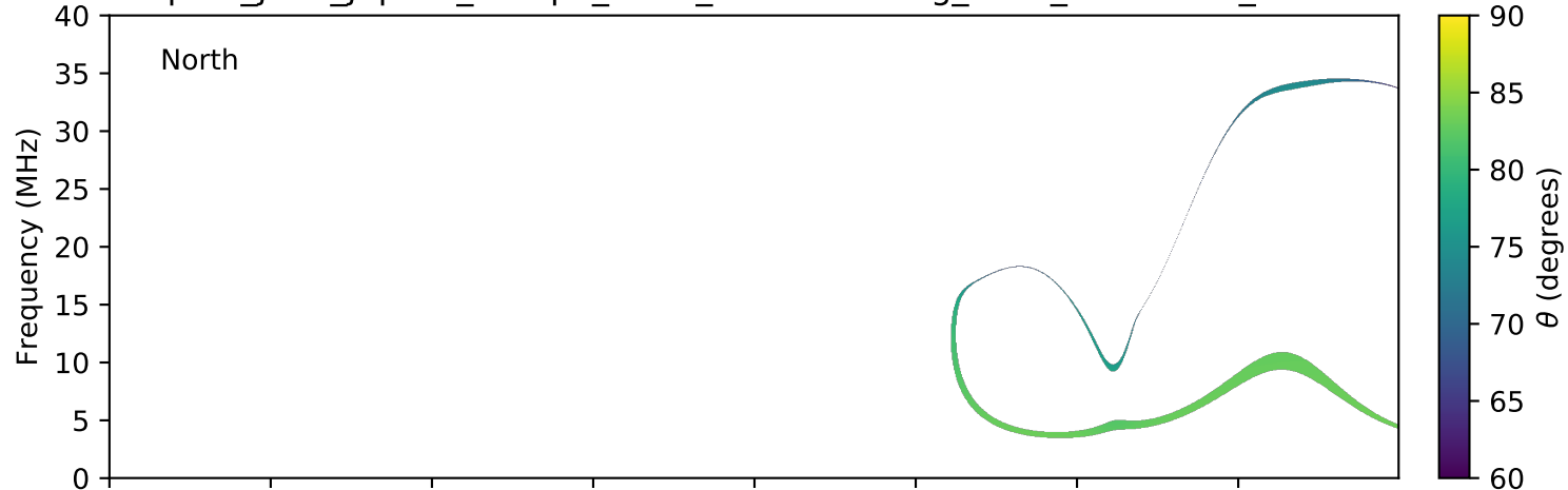
expres_juno_jupiter_europa_isaac_lossc-wid1deg_3kev_20160704_v01.cdf
