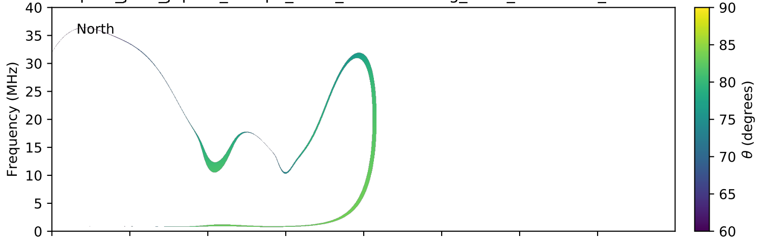
expres_juno_jupiter_europa_isaac_lossc-wid1deg_3kev_20160703_v01.cdf
