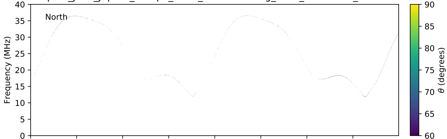
expres_juno_jupiter_europa_isaac_lossc-wid1deg_3kev_20160702_v01.cdf
