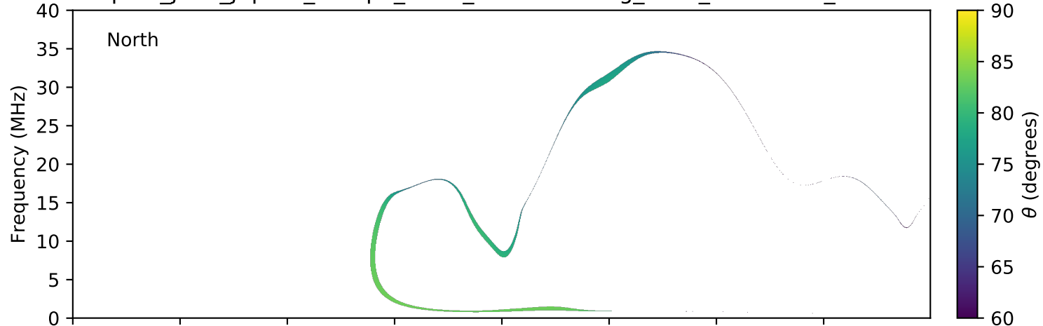
expres_juno_jupiter_europa_isaac_lossc-wid1deg_3kev_20160701_v01.cdf
