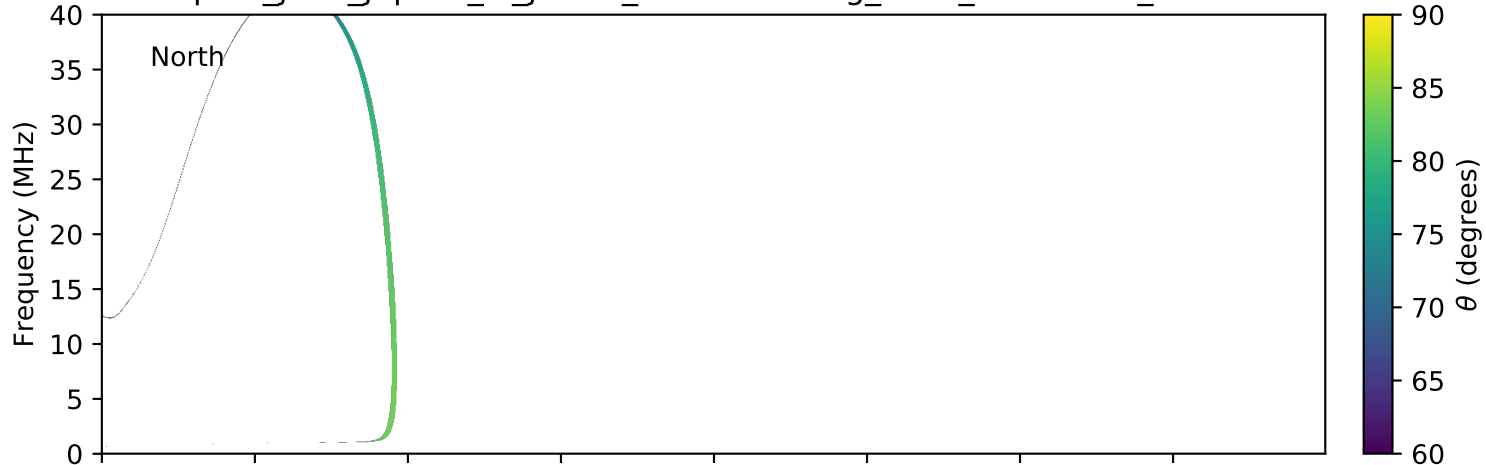
expres_juno_jupiter_io_jrm09_lossc-wid1deg_3kev_20160530_v01.cdf
