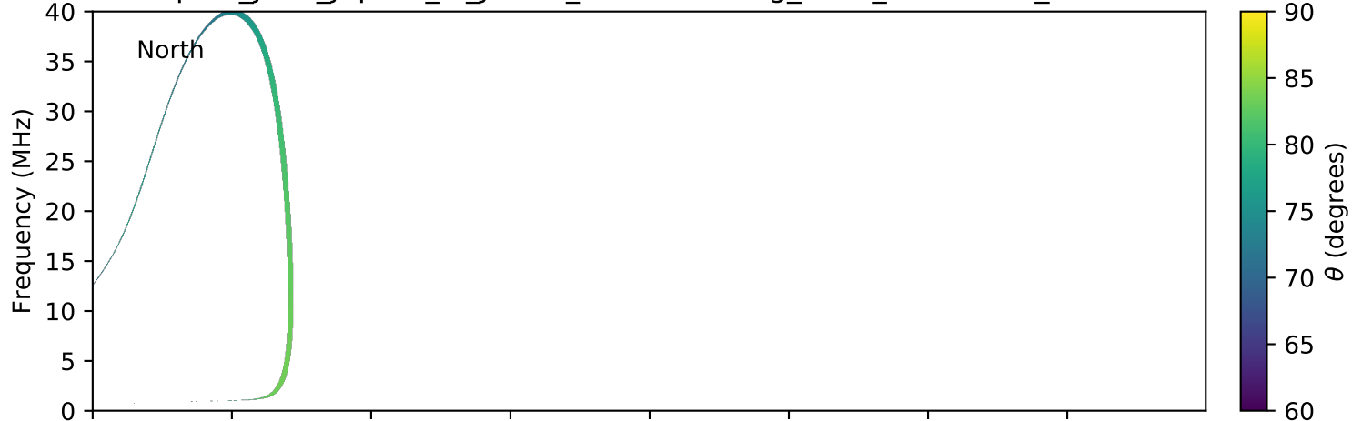
expres_juno_jupiter_io_jrm09_lossc-wid1deg_3kev_20160523_v01.cdf
