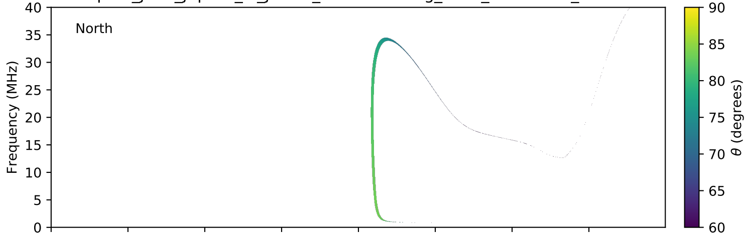
expres_juno_jupiter_io_jrm09_lossc-wid1deg_3kev_20160520_v01.cdf
