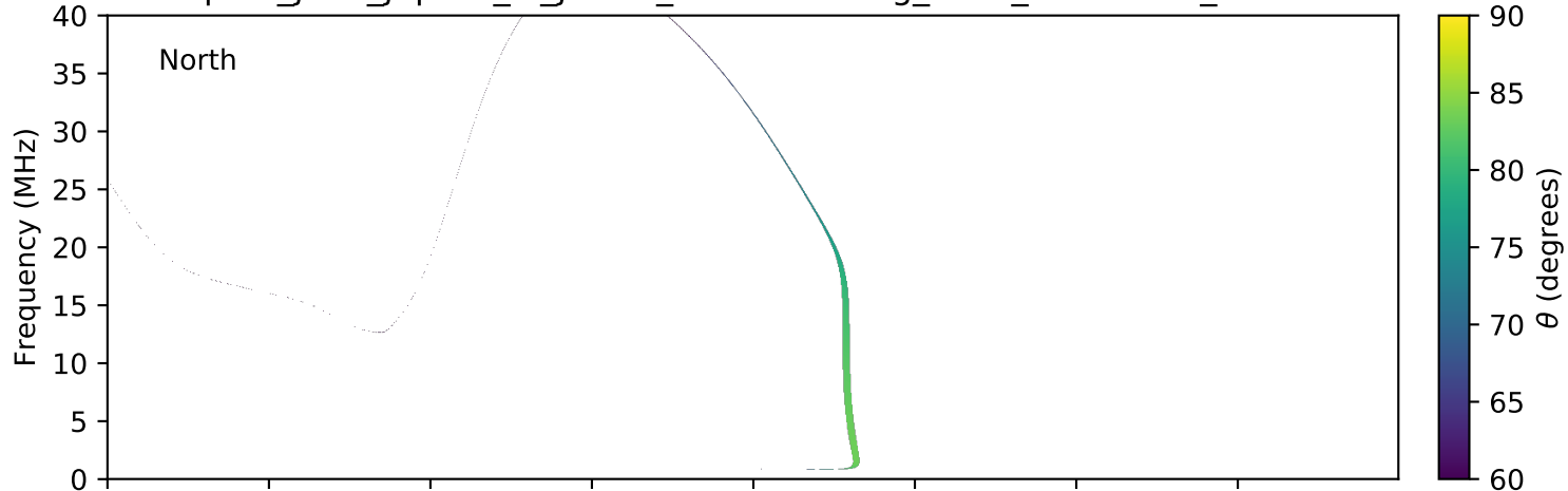
expres_juno_jupiter_io_jrm09_lossc-wid1deg_3kev_20160519_v01.cdf
