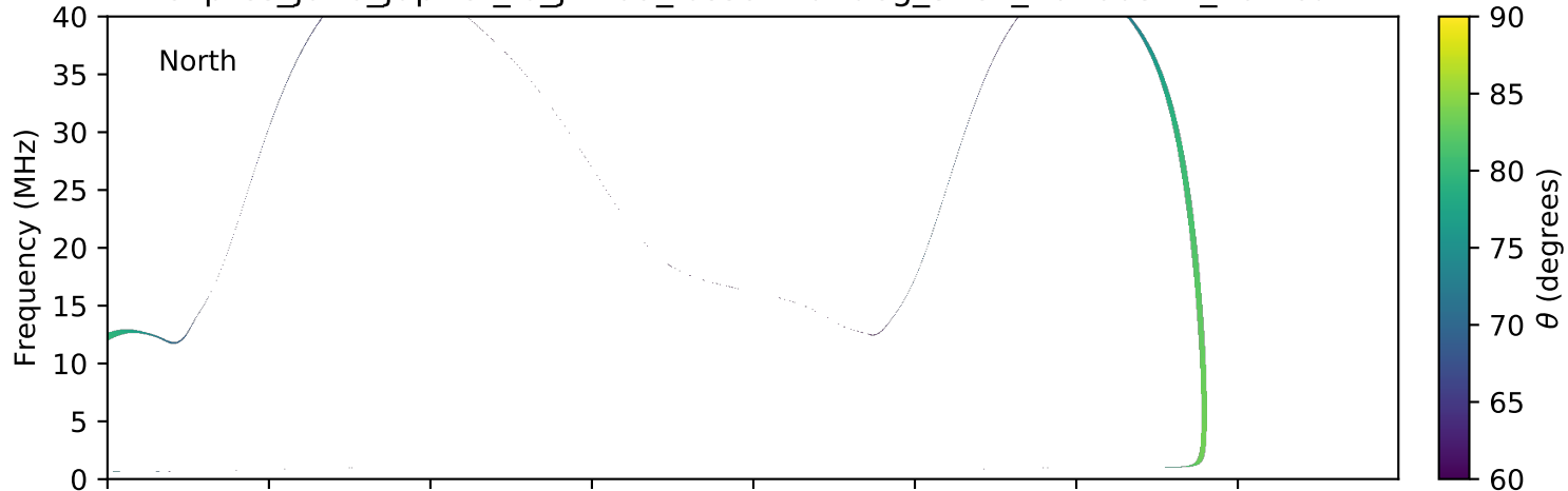
expres_juno_jupiter_io_jrm09_lossc-wid1deg_3kev_20160517_v01.cdf
