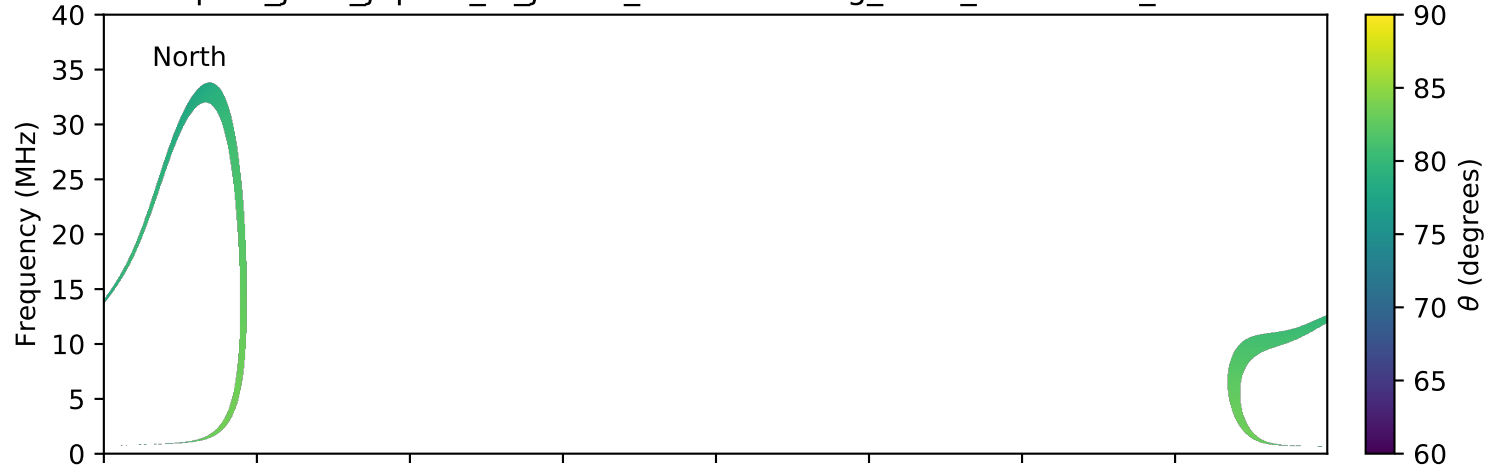
expres_juno_jupiter_io_jrm09_lossc-wid1deg_3kev_20160516_v01.cdf
