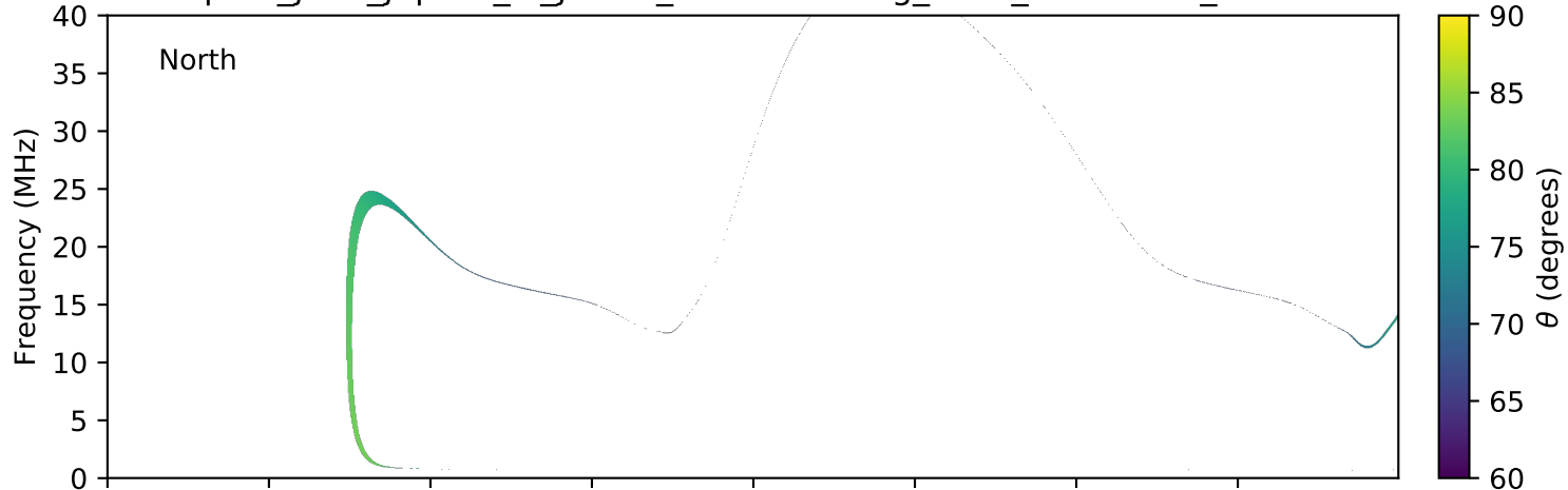
expres_juno_jupiter_io_jrm09_lossc-wid1deg_3kev_20160515_v01.cdf
