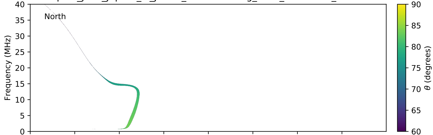
expres_juno_jupiter_io_jrm09_lossc-wid1deg_3kev_20160514_v01.cdf
