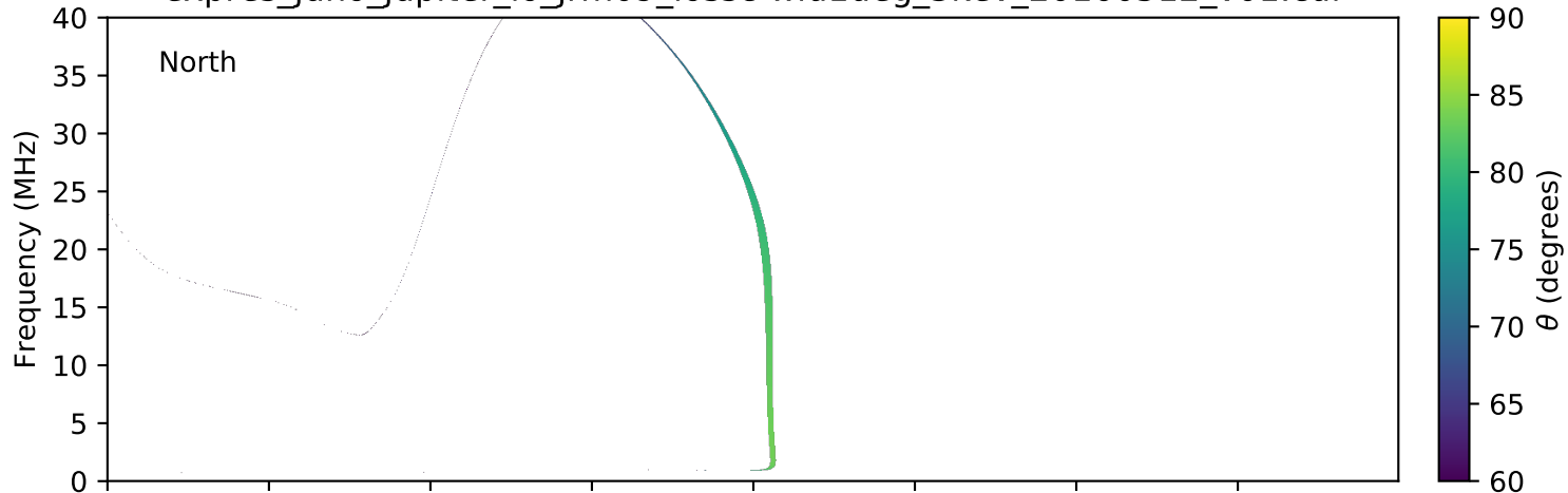
expres_juno_jupiter_io_jrm09_lossc-wid1deg_3kev_20160512_v01.cdf
