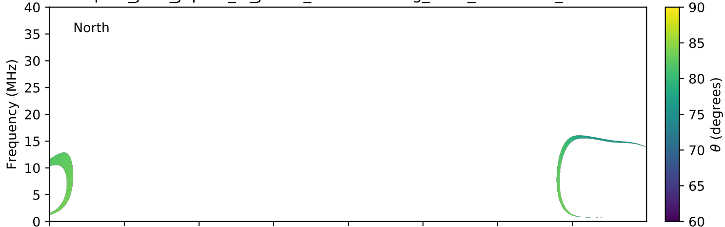
expres_juno_jupiter_io_jrm09_lossc-wid1deg_3kev_20160509_v01.cdf
