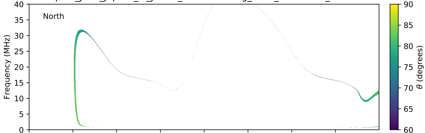
expres_juno_jupiter_io_jrm09_lossc-wid1deg_3kev_20160508_v01.cdf
