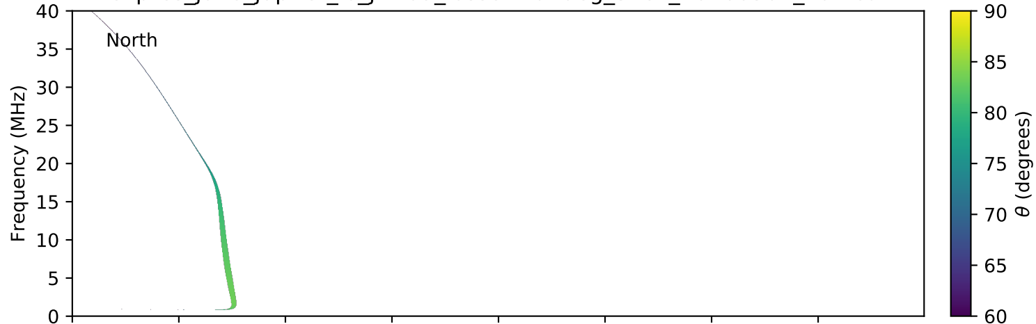
expres_juno_jupiter_io_jrm09_lossc-wid1deg_3kev_20160507_v01.cdf
