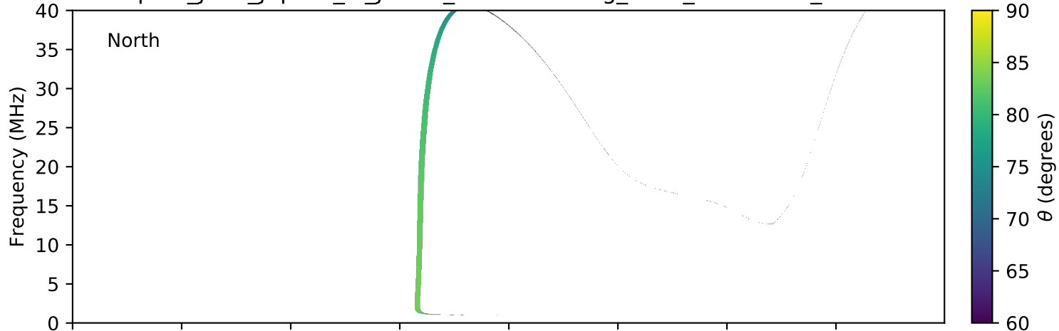
expres_juno_jupiter_io_jrm09_lossc-wid1deg_3kev_20160506_v01.cdf
