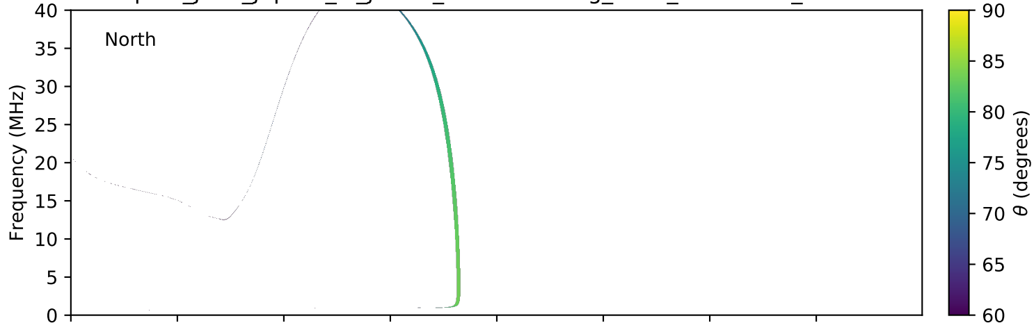
expres_juno_jupiter_io_jrm09_lossc-wid1deg_3kev_20160505_v01.cdf
