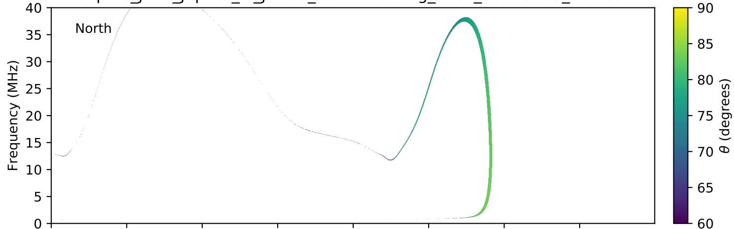
expres_juno_jupiter_io_jrm09_lossc-wid1deg_3kev_20160503_v01.cdf
