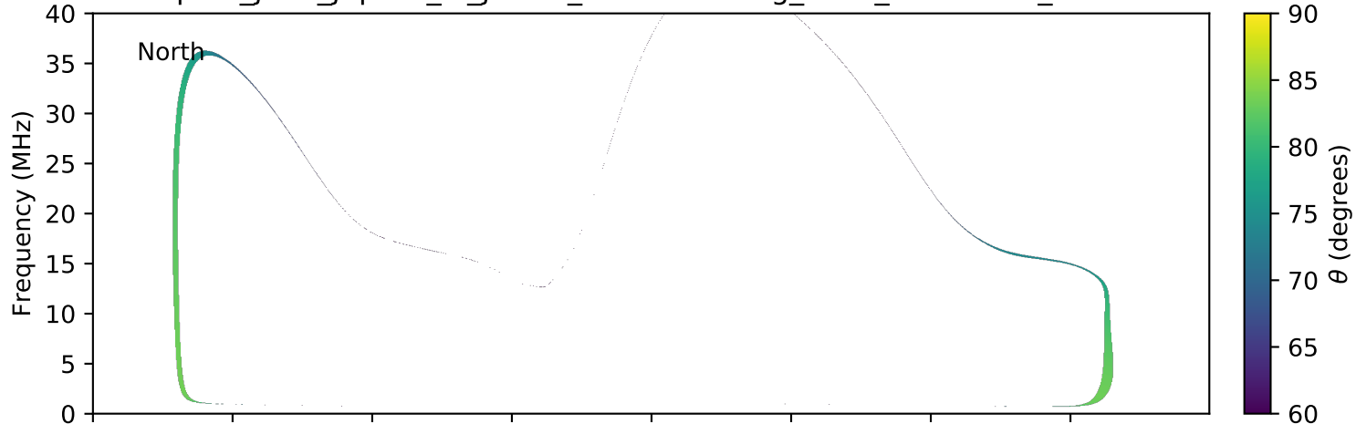
expres_juno_jupiter_io_jrm09_lossc-wid1deg_3kev_20160501_v01.cdf
