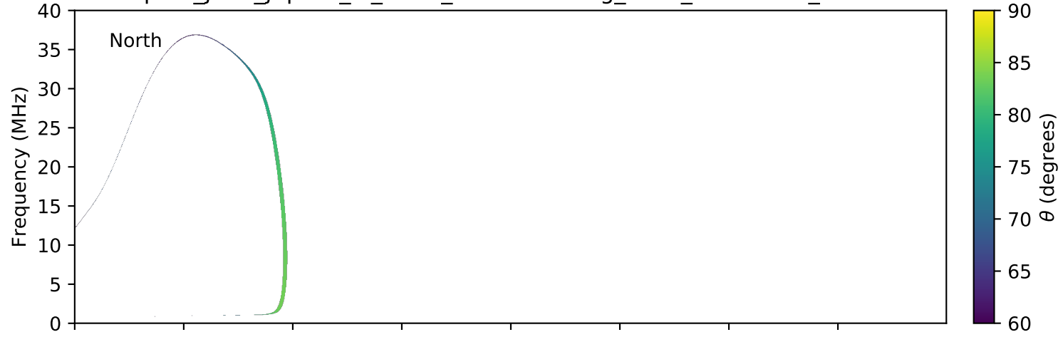
expres_juno_jupiter_io_isaac_lossc-wid1deg_3kev_20160530_v01.cdf
