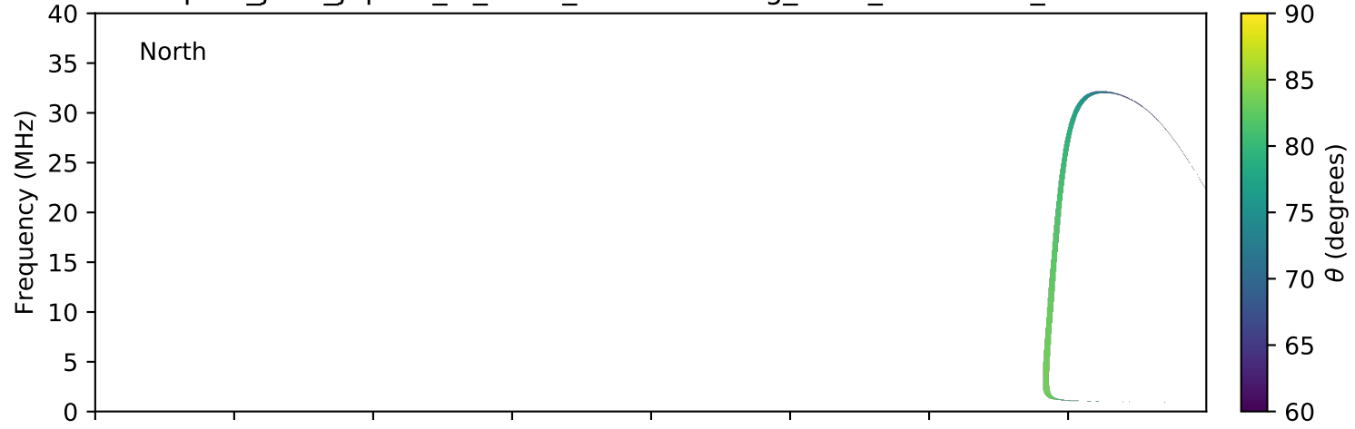
expres_juno_jupiter_io_isaac_lossc-wid1deg_3kev_20160525_v01.cdf
