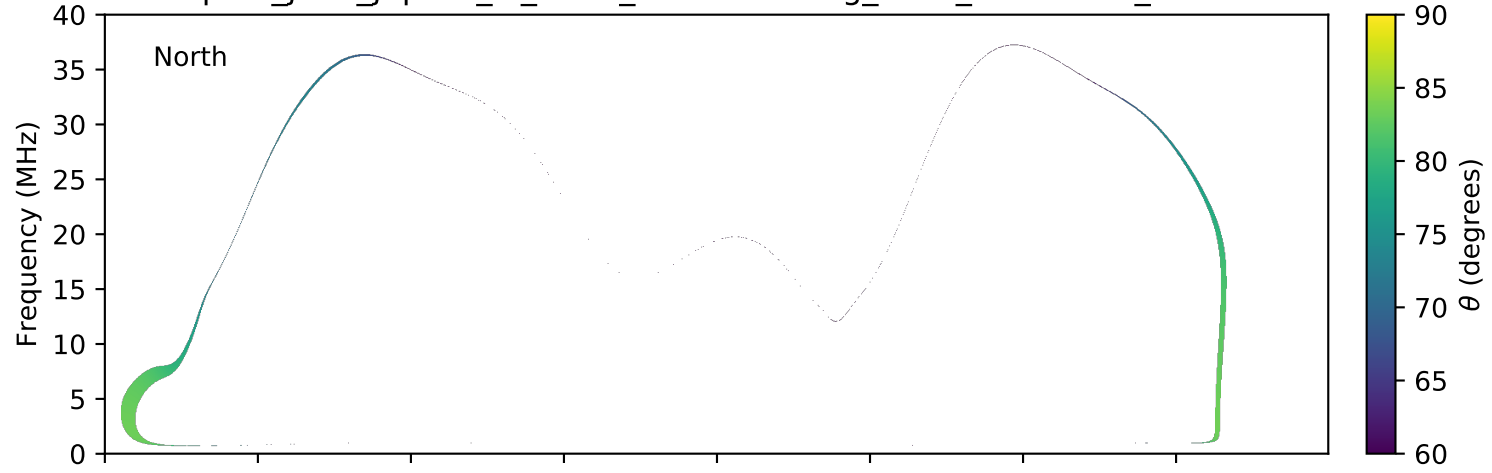
expres_juno_jupiter_io_isaac_lossc-wid1deg_3kev_20160524_v01.cdf
