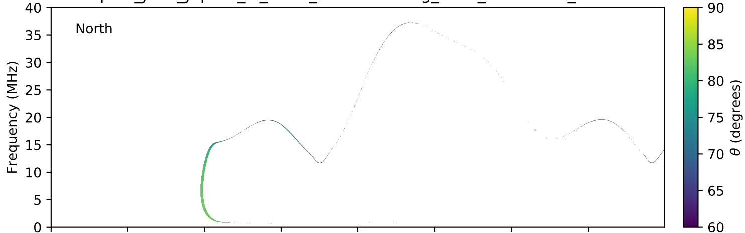
expres_juno_jupiter_io_isaac_lossc-wid1deg_3kev_20160522_v01.cdf
