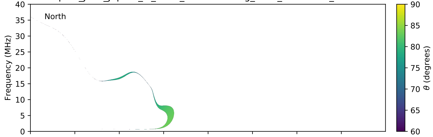
expres_juno_jupiter_io_isaac_lossc-wid1deg_3kev_20160521_v01.cdf
