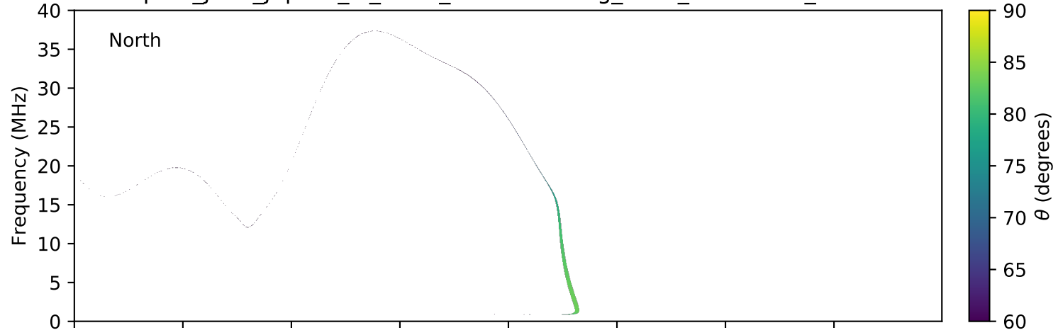
expres_juno_jupiter_io_isaac_lossc-wid1deg_3kev_20160519_v01.cdf
