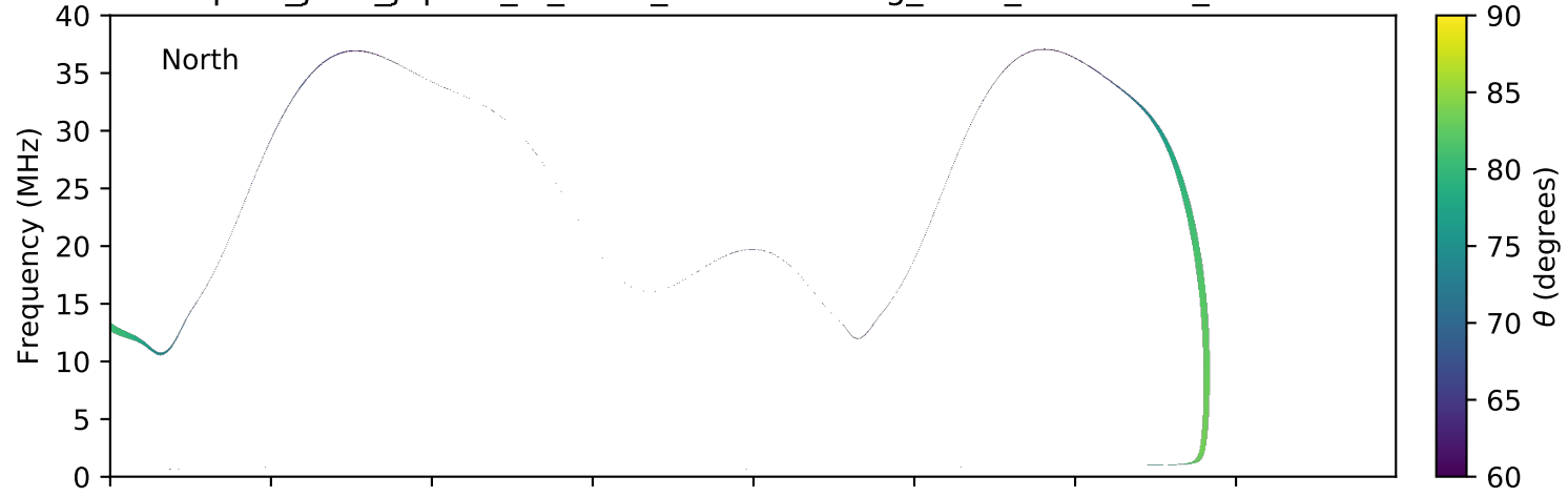
expres_juno_jupiter_io_isaac_lossc-wid1deg_3kev_20160517_v01.cdf
