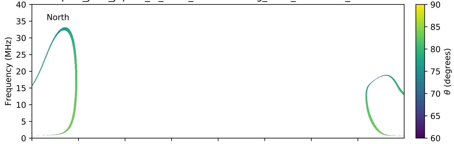
expres_juno_jupiter_io_isaac_lossc-wid1deg_3kev_20160516_v01.cdf
