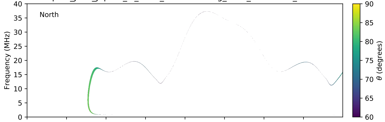
expres_juno_jupiter_io_isaac_lossc-wid1deg_3kev_20160515_v01.cdf
