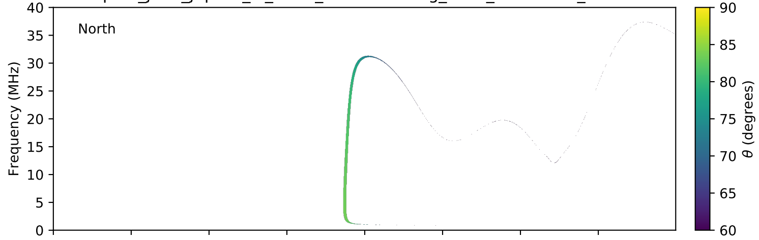
expres_juno_jupiter_io_isaac_lossc-wid1deg_3kev_20160513_v01.cdf
