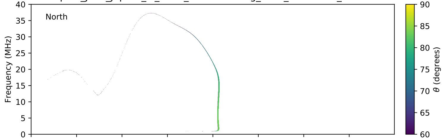
expres_juno_jupiter_io_isaac_lossc-wid1deg_3kev_20160512_v01.cdf
