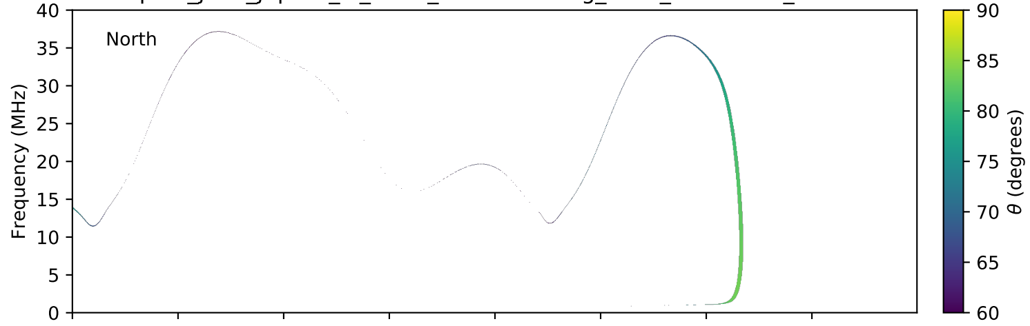
expres_juno_jupiter_io_isaac_lossc-wid1deg_3kev_20160510_v01.cdf
