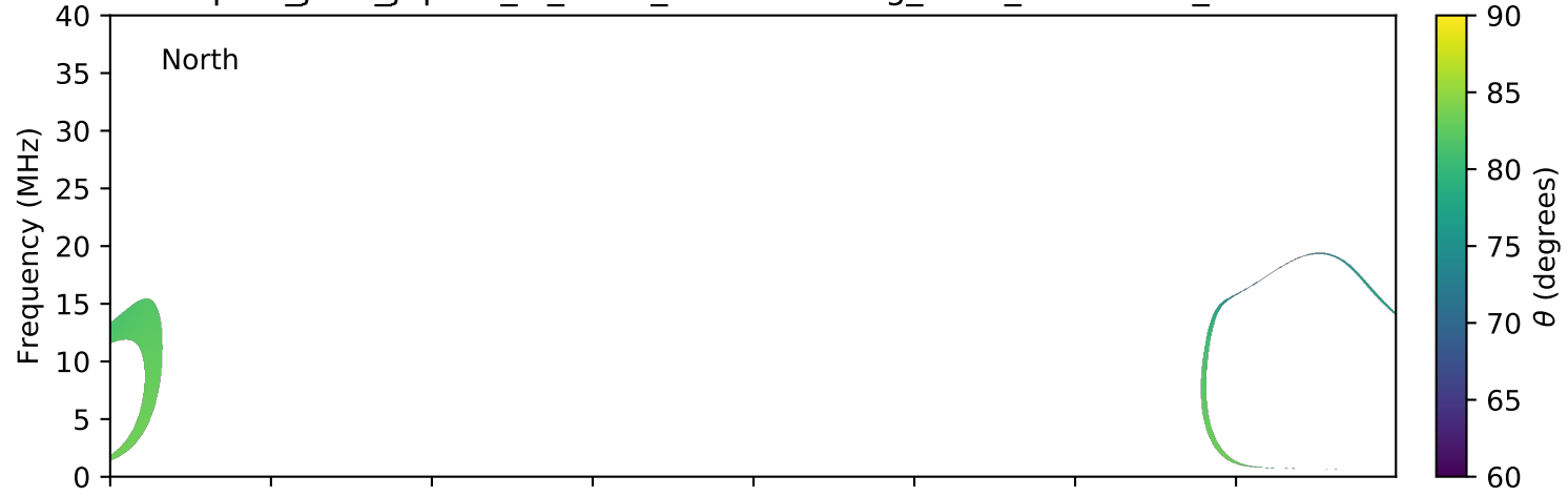
expres_juno_jupiter_io_isaac_lossc-wid1deg_3kev_20160509_v01.cdf
