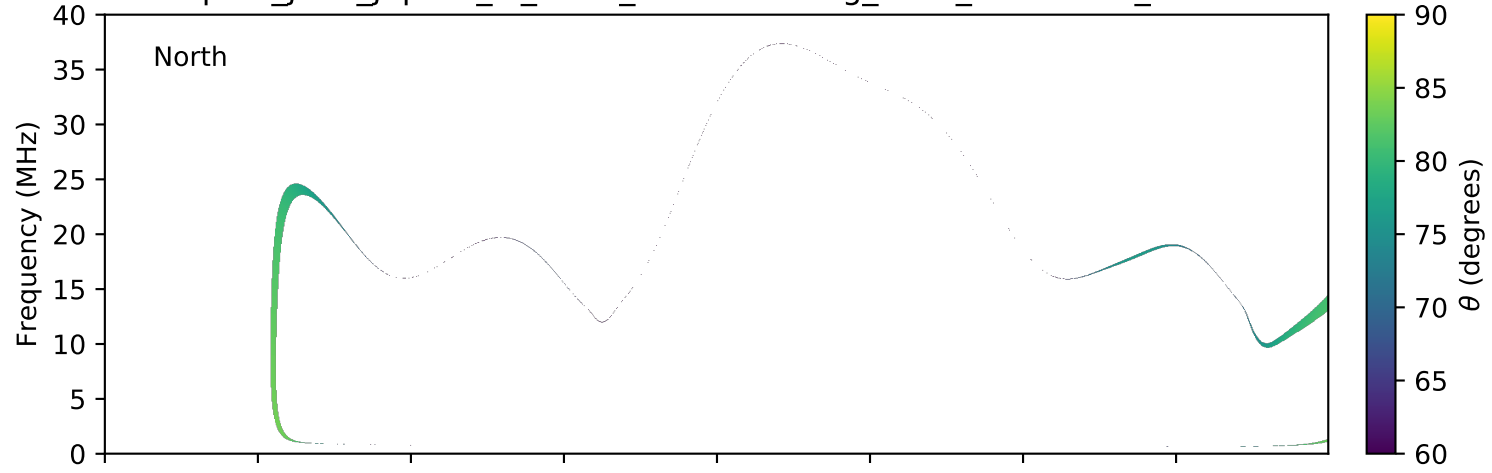
expres_juno_jupiter_io_isaac_lossc-wid1deg_3kev_20160508_v01.cdf
