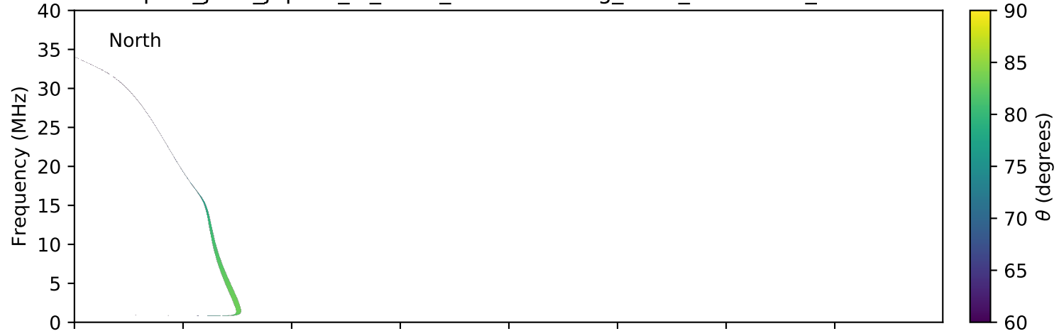
expres_juno_jupiter_io_isaac_lossc-wid1deg_3kev_20160507_v01.cdf
