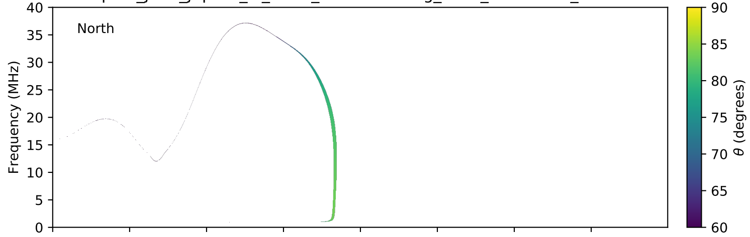
expres_juno_jupiter_io_isaac_lossc-wid1deg_3kev_20160505_v01.cdf
