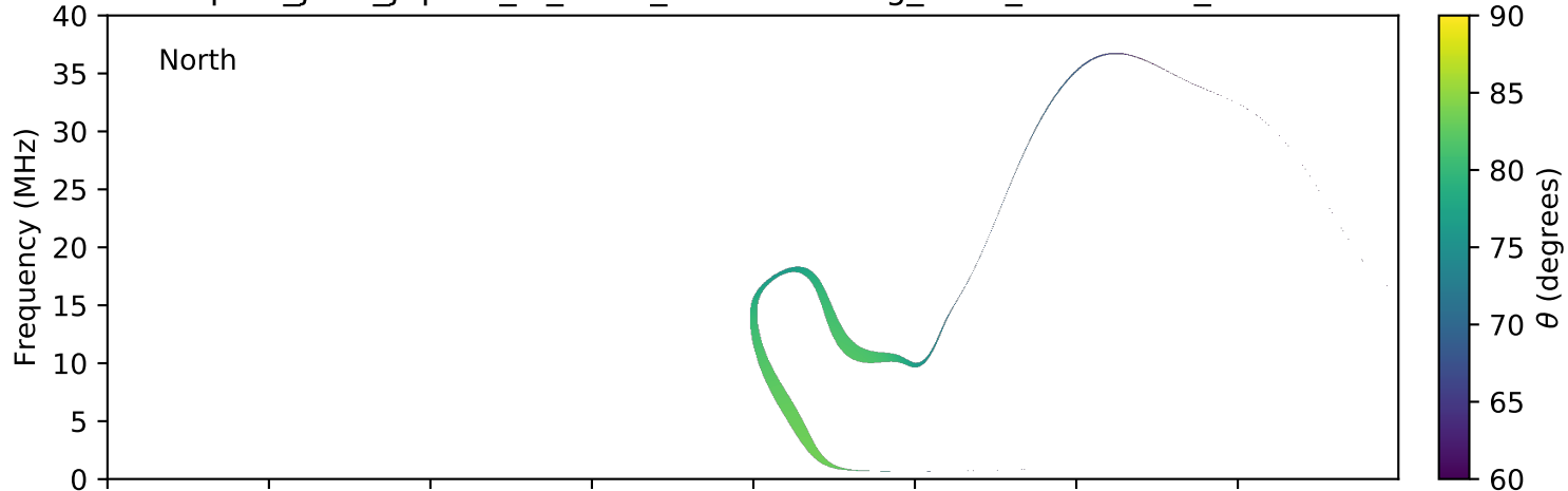
expres_juno_jupiter_io_isaac_lossc-wid1deg_3kev_20160504_v01.cdf
