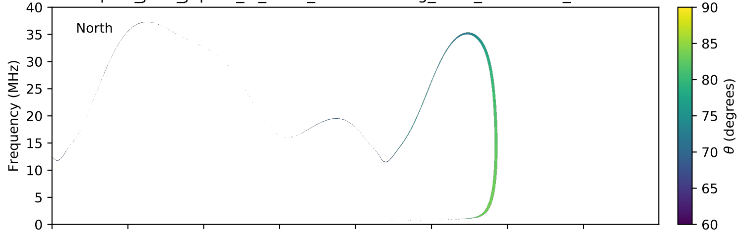
expres_juno_jupiter_io_isaac_lossc-wid1deg_3kev_20160503_v01.cdf
