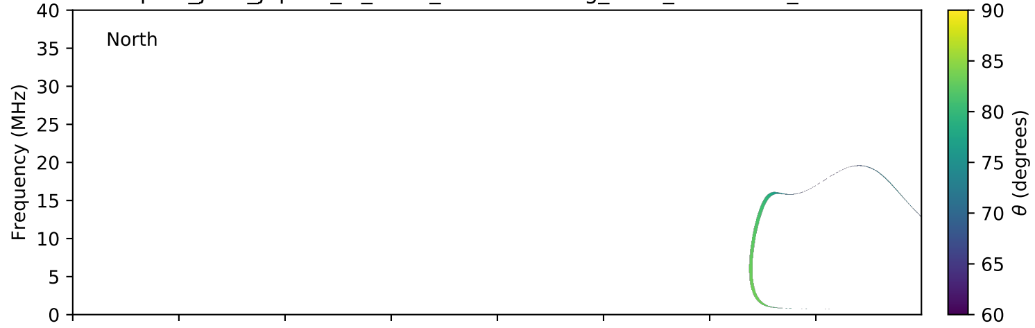
expres_juno_jupiter_io_isaac_lossc-wid1deg_3kev_20160502_v01.cdf
