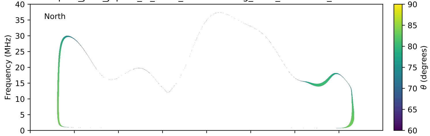
expres_juno_jupiter_io_isaac_lossc-wid1deg_3kev_20160501_v01.cdf
