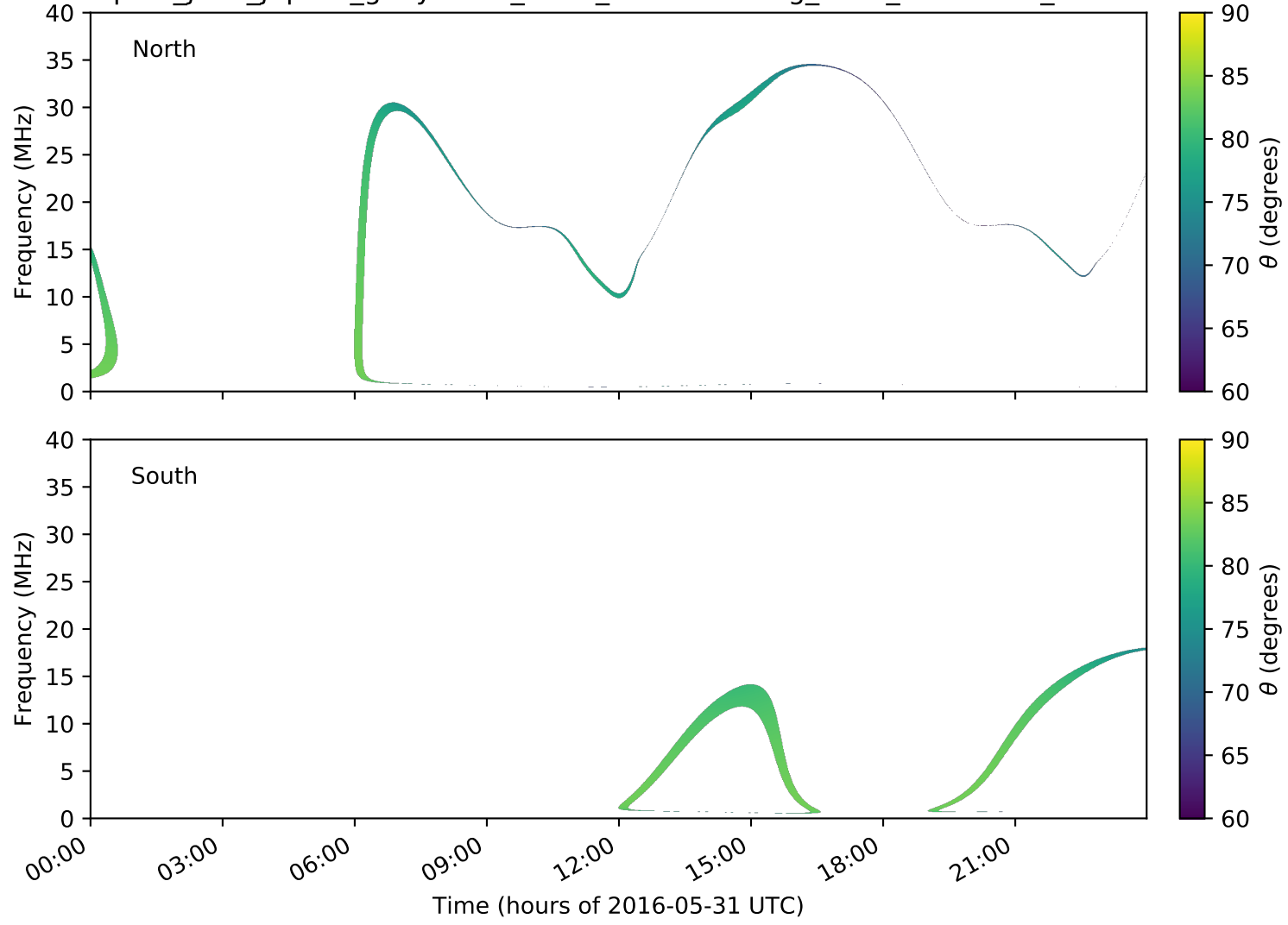
expres_juno_jupiter_ganymede_isaac_lossc-wid1deg_3kev_20160531_v01.cdf
